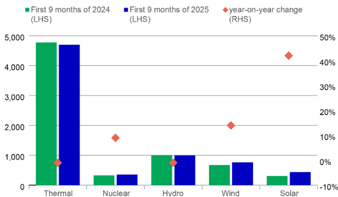
Chart 2: Chinese mainland's power generation (billion kWh)
